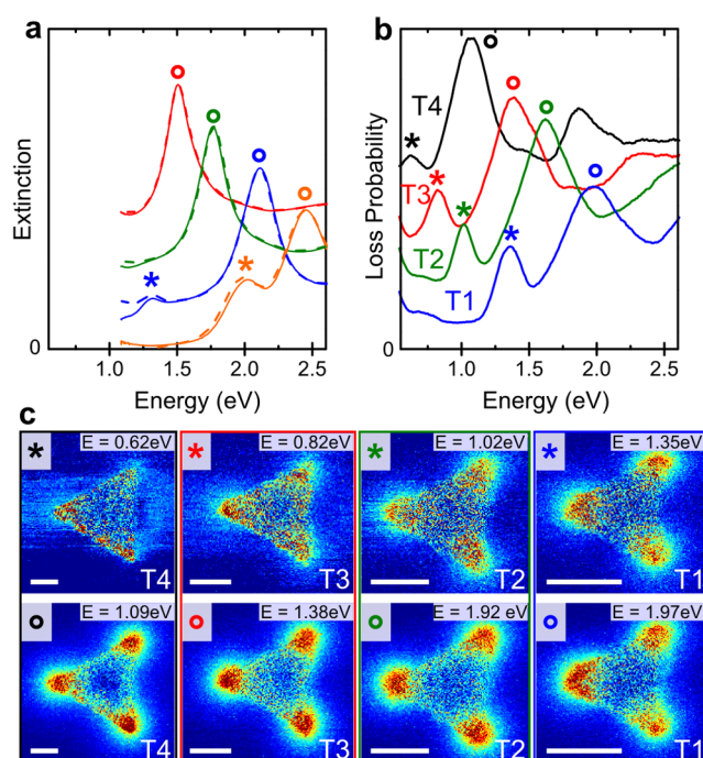
Figure 2. Dipole resonances on 3D dimers: (a) Optical extinction spectra of four 3D dimers. The two orthogonal polarizations (horizontal and vertical with respect to the triangle orientation in c) are shown by the solid and dashed (mostly overlapping) lines. For the two smaller 3D dimers (blue and orange lines) two resonance peaks are visible (labeled * and O); for the larger 3D dimers (green and red lines) the low energy peak (*) shifts out of the range of the spectrometer. (b) EELS spectra summed over the full spectrum images taken from T1 to T4 showing two resonance peaks (* and O) for all dimers, colors indicate particles of approximately same size. (c) 2D EELS maps extracted from the peak positions indicated in panel b. Curves in a and b are bare shifted by a constant offset relative to orange and blue curves, respectively. Scale bars are 100 nm.
