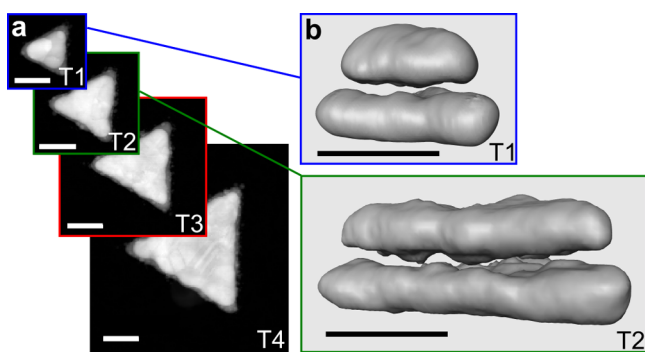
Figure 1. Morphology of 3D dimers: (a) HAADF STEM images of four silver 3D dimers of different sizes, labeled T1 to T4 with increasing size. (b) 3D reconstructions of the two smallest dimers T1 and T2. Scale bars are 100 nm.
