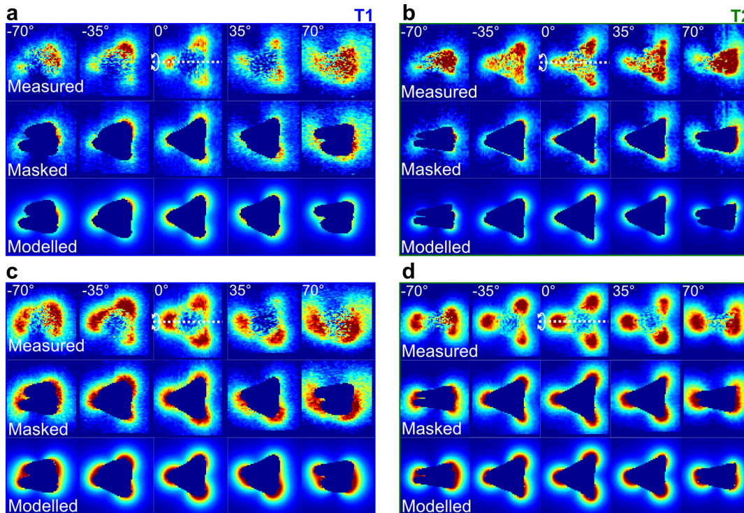
Figure 3. Comparison of measured and reprojected (modeled) EELS maps for five tilt angles as indicated, for the low-energy dipole mode (bonding) on (a) the dimer T1 and (b) the dimer T2 and for the high energy dipole mode (antibonding) on (c) T1 and (d) T2. For each mode the top row shows the measured (zero-loss normalized and deconvolved) data. The second row shows only data points at least 5 nm away from the particle, which are taken into account for the reconstruction. The lowest row shows the modeled (reprojected) maps, which result from the reconstruction. In the 0° projections the tilt axis is indicated.
