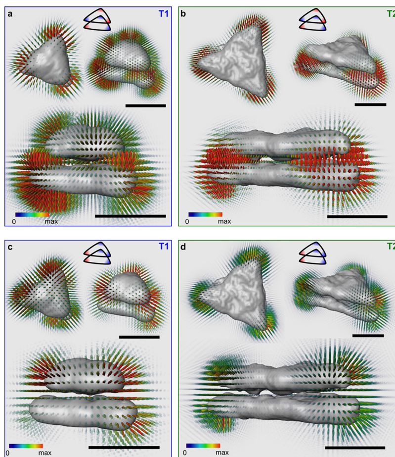
Figure 4. 3D reconstruction of the photonic LDOS: (a) Low-energy (bonding) mode of the dimer T1 and (b) T2. (c) High-energy (antibonding) mode of the dimer T1 and (d) T2. The orientation of the pencils indicates the direction along which the LDOS is maximal. Color, transparency, and length correspond to the magnitude of the full LDOS. The same color scale range is used for all modes to allow a relative comparison of their LDOS magnitude. The insets schematically show the charge distributions of the bonding and antibonding modes. Scale bars are 100 nm.
